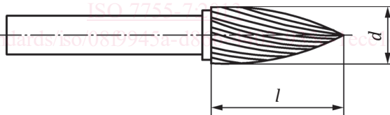
Figure 1 — Hardmetal burr, style G
