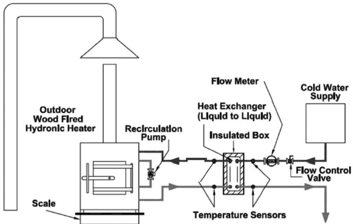
FIG. 2 Set-Up Schematic
