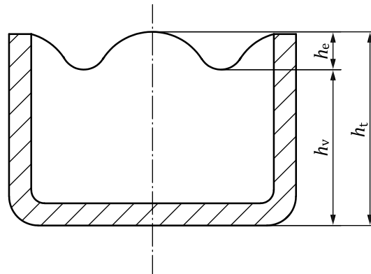
Figure 1 — Schematic section of cup
