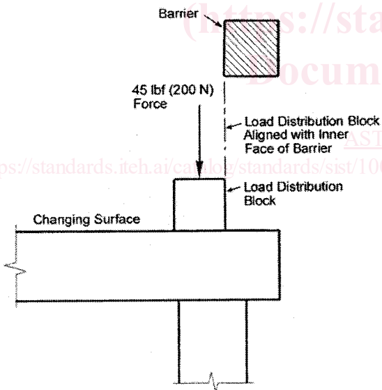
FIG. 3 Stability Test
