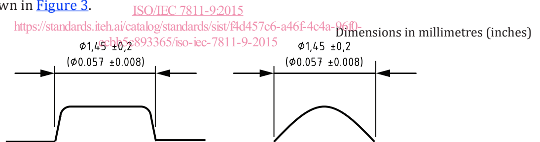
Figure 3 — TIM dot base size and shape illustration
