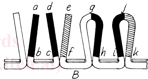
ad = cut pile tuft element gj = loop pile tuft element ab, cd, ef, gh, ij, jk = tuft legs cd, ef = cut pile tuft leg pair ij, jk = loop pile tuft leg pair, a loop B = one binding site
