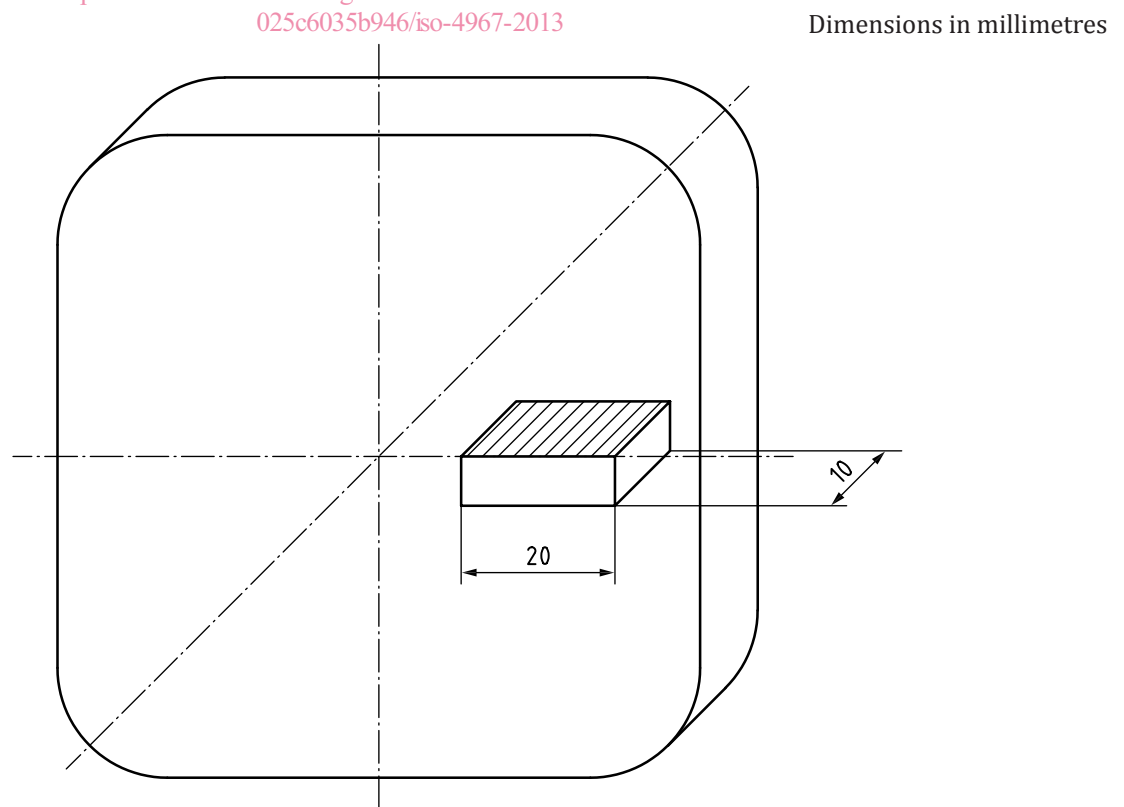
Figure 1 — Sample from bar or billet with a diameter or length of side > 40 mm
