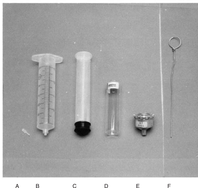
FIG.-2 3 Test Supplies and Accessory
