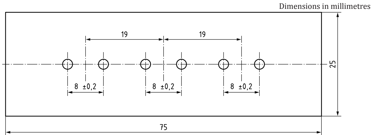
Figure 1 — Test piece
