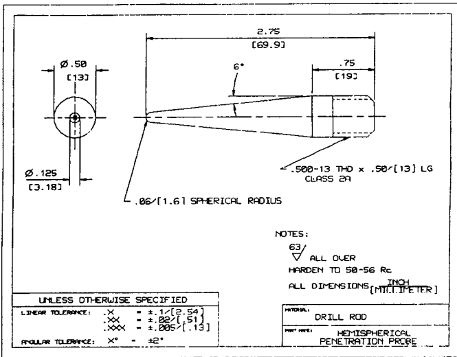
FIG. 1 Penetration Probe
