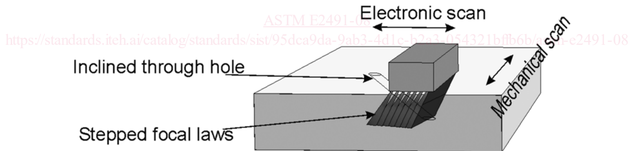
FIG. A1.5 Representation of an Inclined Hole for Beam Characterization in the Passive Plane
