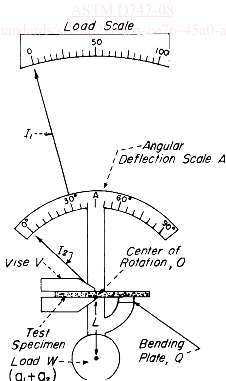
FIG. 1 Mechanical System of Test Apparatus
