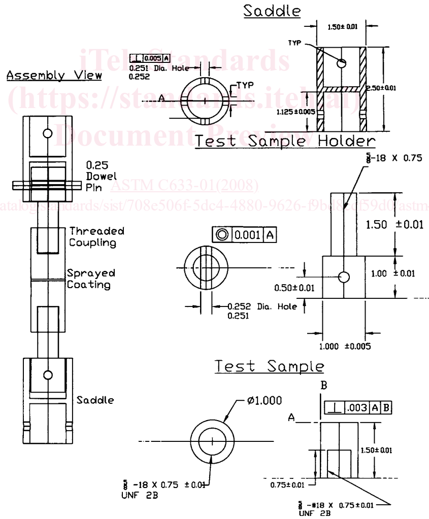
FIG. 1 Self-Aligning Device
