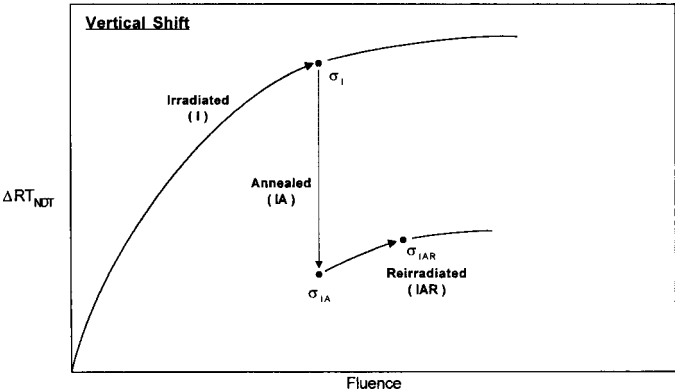
FIG. X2.2 Vertical Shift Method for Estimating Reirradiation Embrittlement
