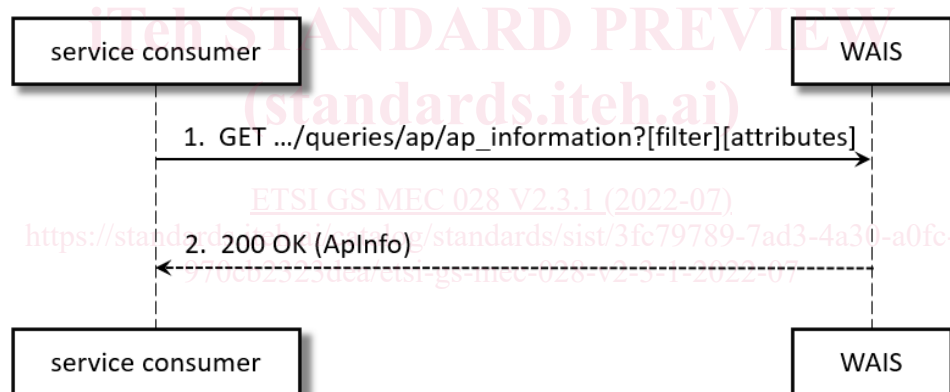
Figure 5.2.2.1-1: Flow of service consumer querying Access Point information
