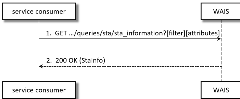
Figure 5.2.3.1-1: Flow of service consumer querying station Info
