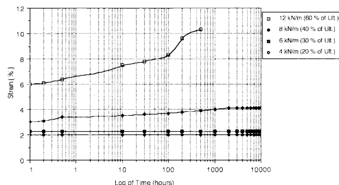
FIG. 1 Percent Strain Versus Log of Time
