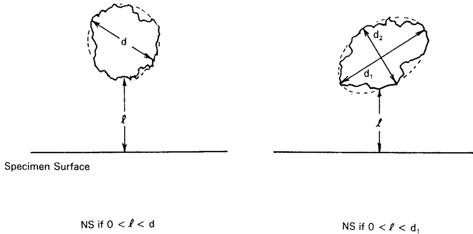
FIG. 6 Schematic Showing Origins and Their Dimensions Relative to the Specimen Surface
