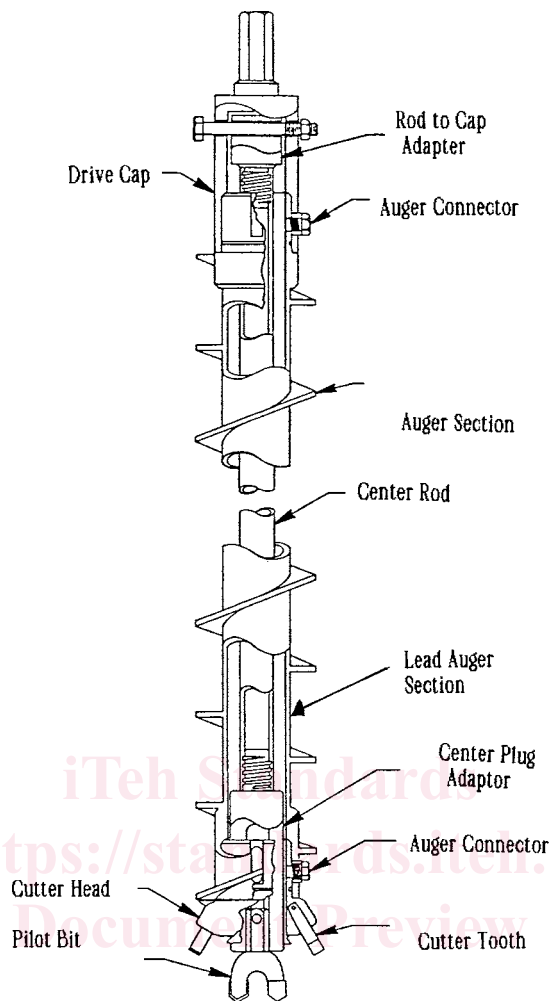
FIG. 1 Rod-Type Auger System With Pilot Bit 5
