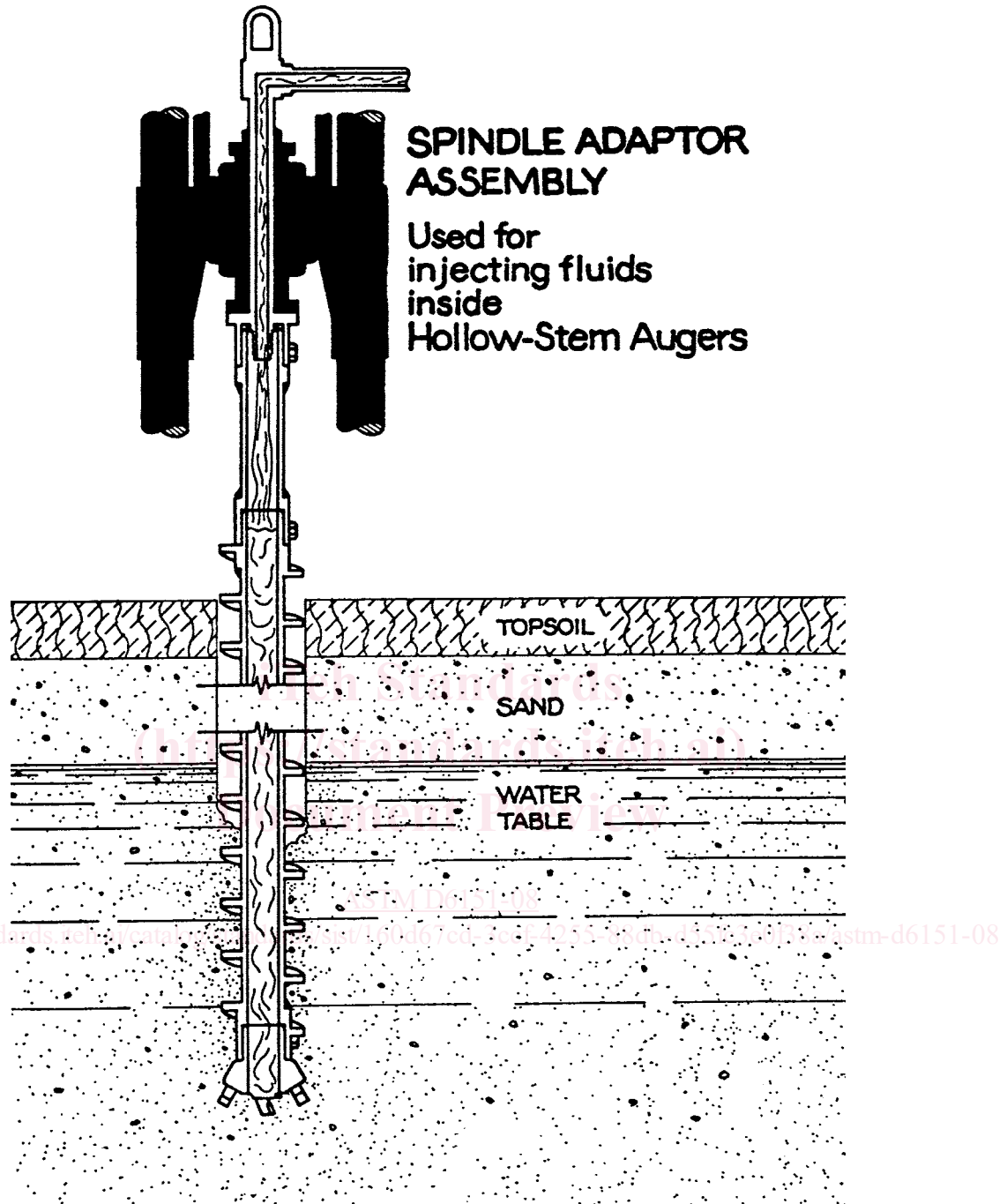
FIG. 4 Spindle Adaptor Assembly
