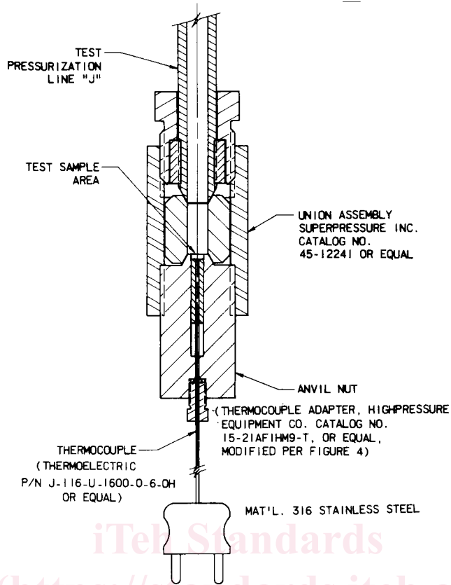
FIG. 3 Test Chamber Subassembly
