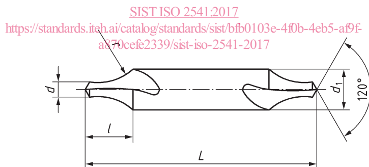
Figure 1 — Centre drills — Type R
