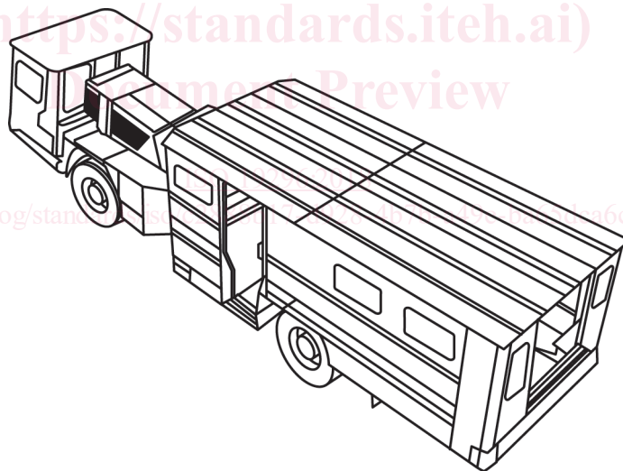
Figure 7 — Personnel transporter
