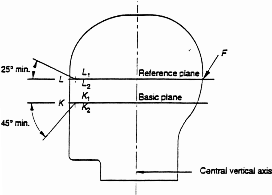
Section of headform in longitudinal vertical plane
