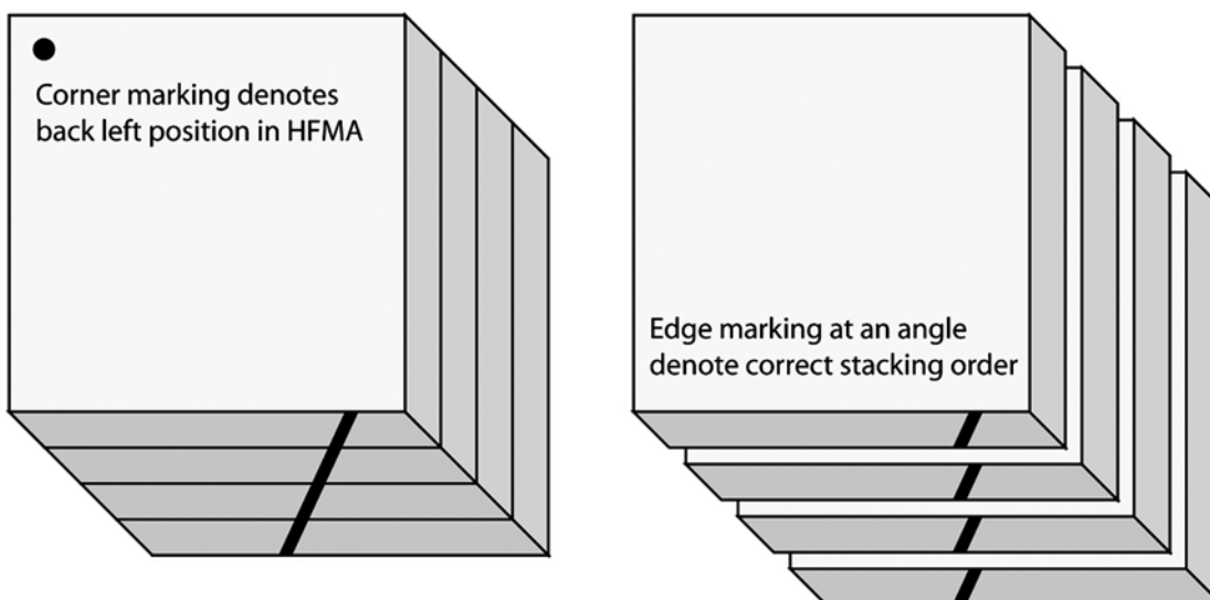
FIG. 3 Examples of Useful Specimen Stack Marking Techniques
