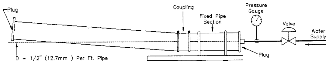
FIG. 1 Deflection Test
