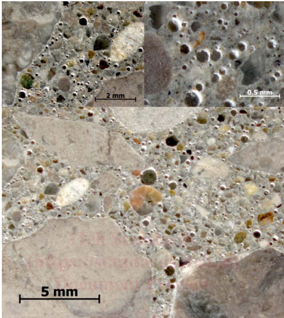
https://standards.iteh.ai/catalog/standards/sist/62951202-2017-astm-c457-08c FIG. 1 Photographs of a Satisfactory Surface
