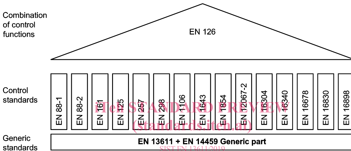
https://standards.iteh.ai/catalog/standards/sist/b028968b-7409-4751-9c76-40024b766c5/sist-en-13611-2019 Figure 1 — Interrelation of control standards
