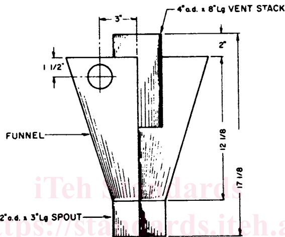
FIG. 2 Cyclone Receiver Weldment
