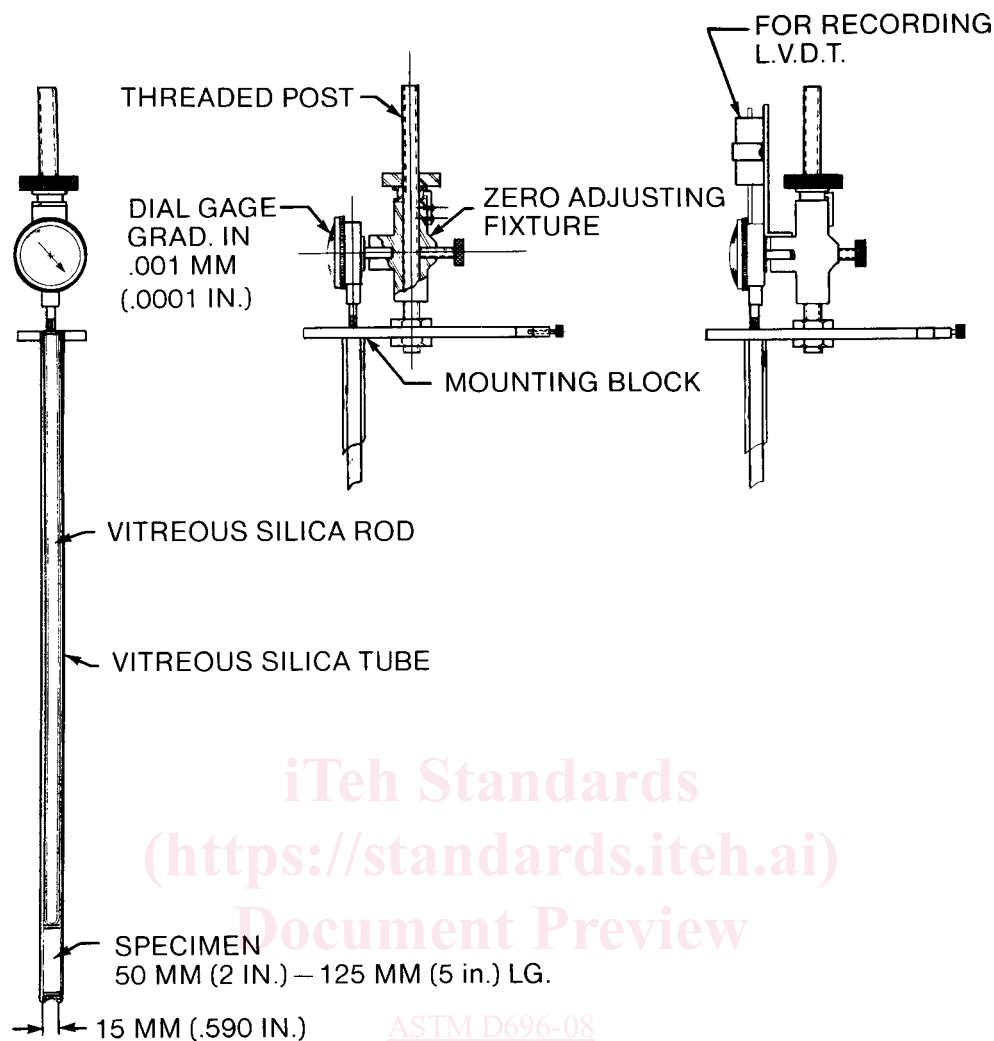
ASTM D696-08 FIG. 1 Quartz-Tube Dilatometer
