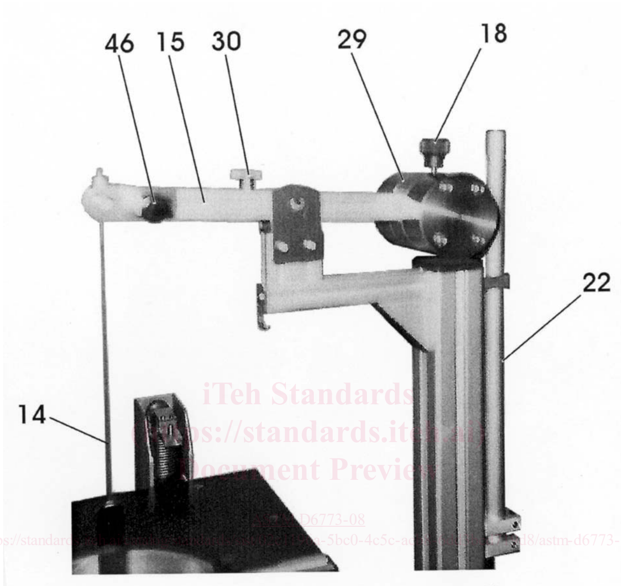
FIG. 6 Counterweight System
