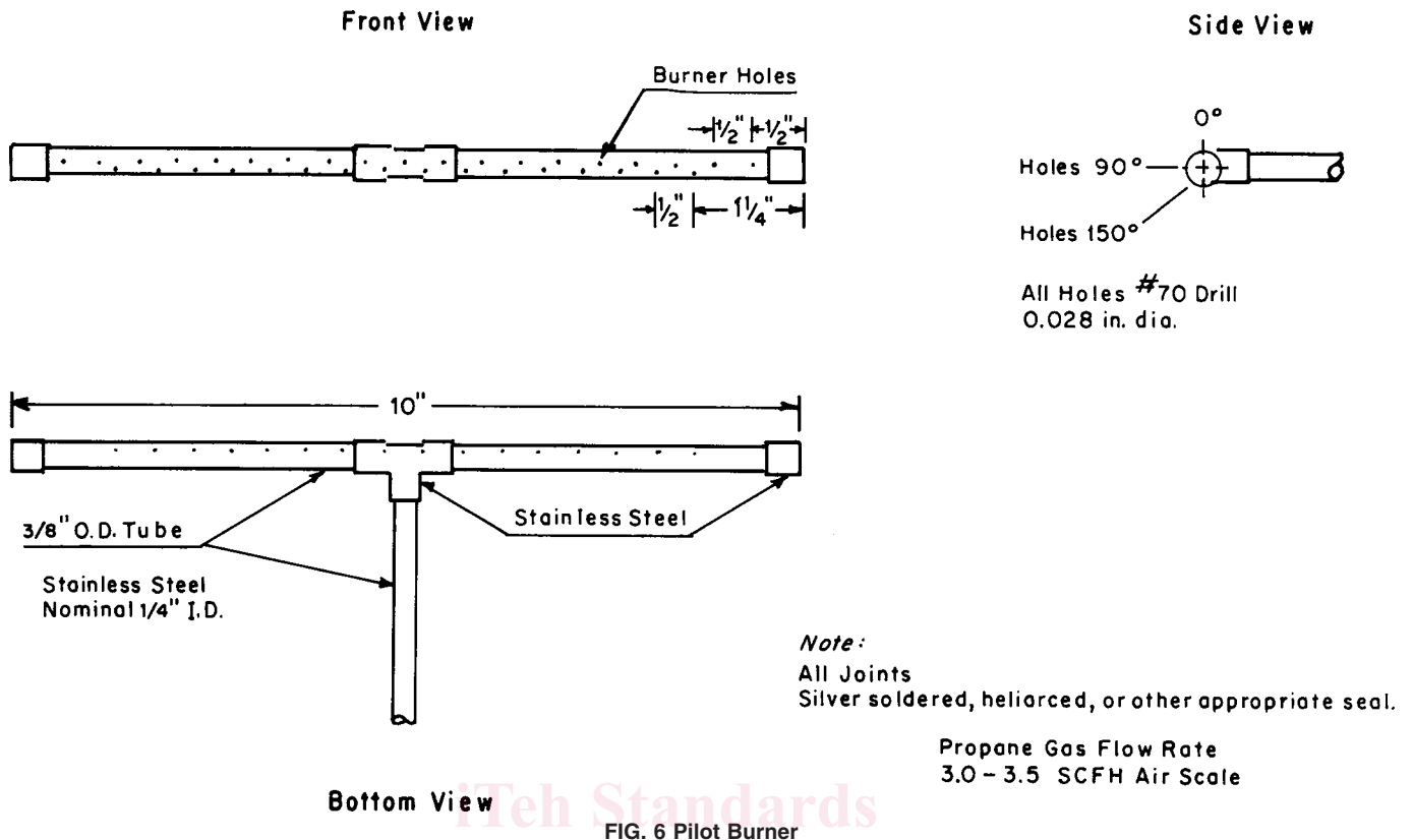
FIG. 6 Pilot Burner
