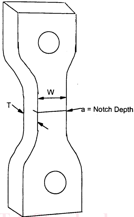
Front view of the notched specimen
