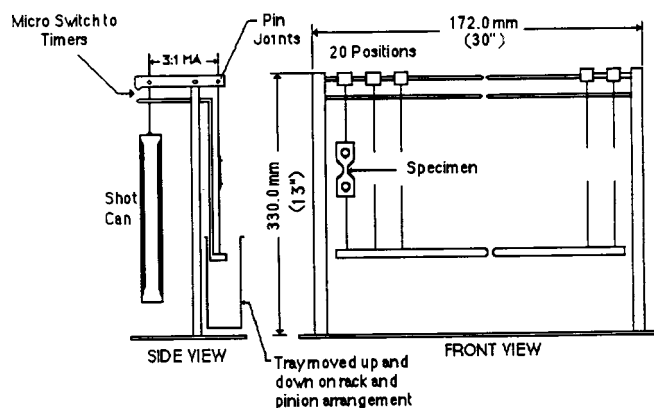
FIG. 2 Constant Stress Loading Apparatus Consisting of Twenty Specimen Test Positions
