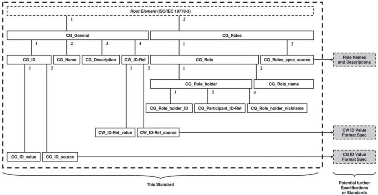
Figure 2 — Collaborative group Data Model and external specifications
