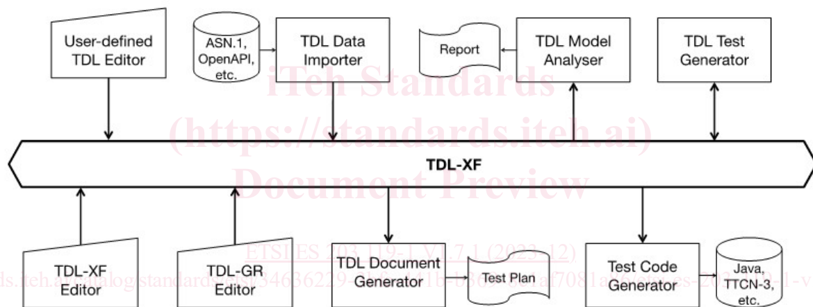
Figure 4.2: A scalable TDL tool architecture
