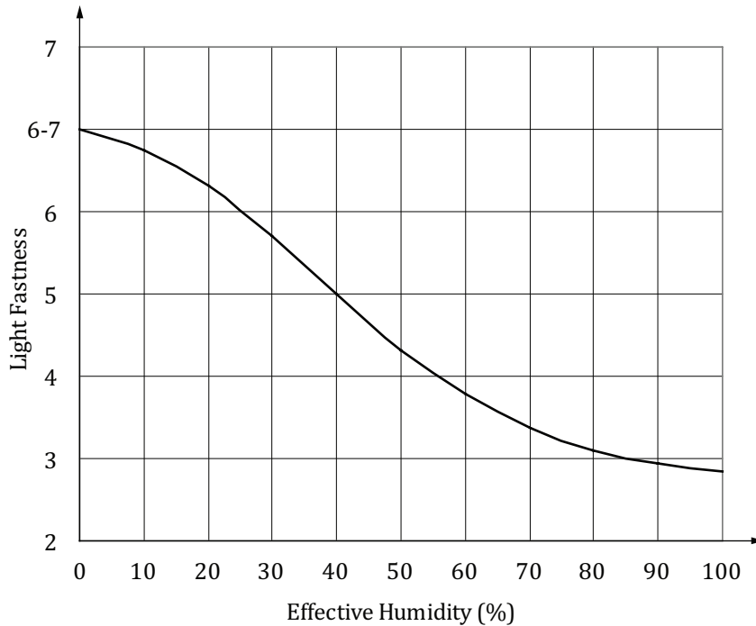
Figure 1 — Mean values obtained from humidity-test control exposures (standards.iteh.ai)
