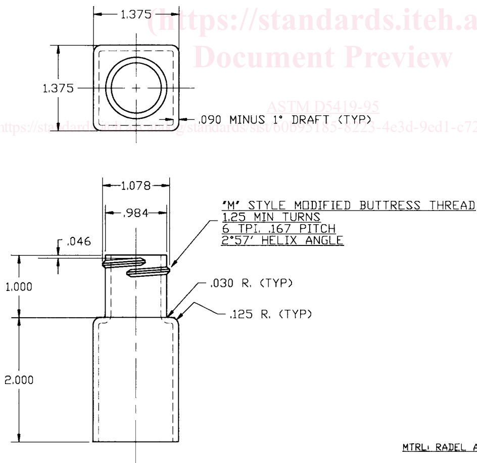
FIG. 1 Typical Fixture
