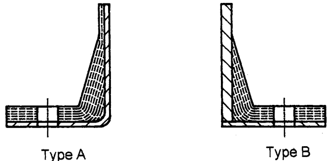
FIG. 1 Flange Types
