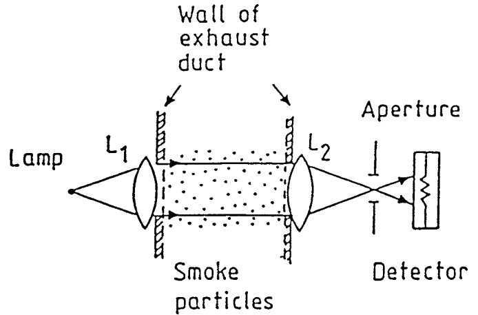
FIG. 3 Optical System
