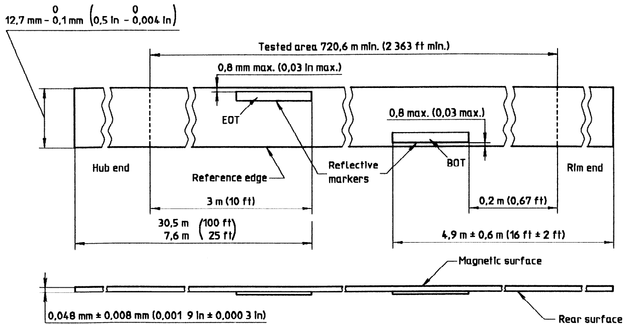
Figure 1 — Tape characteristics iTeh STANDARD PREVIEW (standards.iteh.ai)
