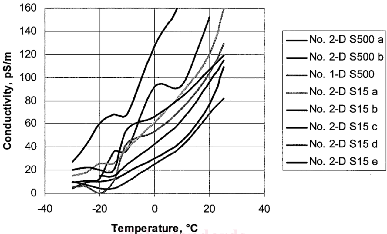
FIG. X1.1 Conductivity Varies with Temperature
