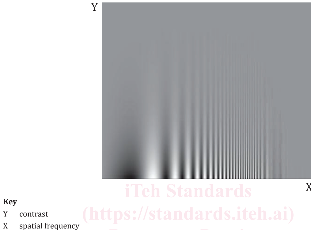
Figure 3 — Illustrative contrast sensitivity function (Reference [3])
