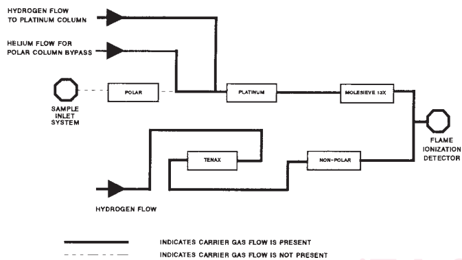
NOTE 1—Polar column is placed in stop flow. FIG. 4 End of the "A" Time
