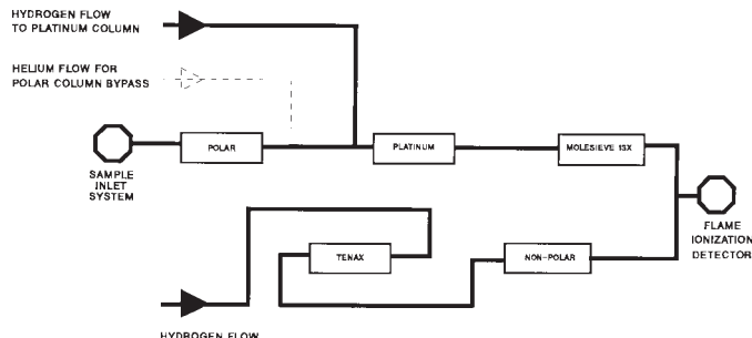
FIG. 12 Final Elution to the Non-Polar Column
