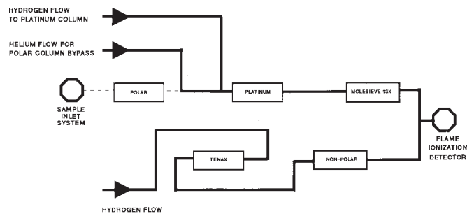
NOTE 1—Begin first aromatic elution to the detector. FIG. 6 End of the "B" Time
