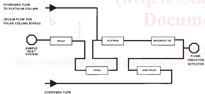
NOTE 1—First aromatic elution from the polar column. FIG. 5 Start of the "B" Time
