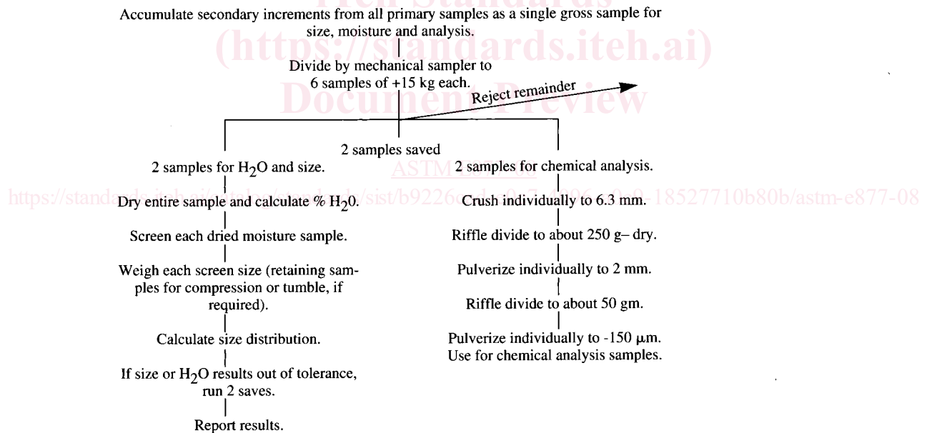
FIG. 3 Flowsheet Examples
