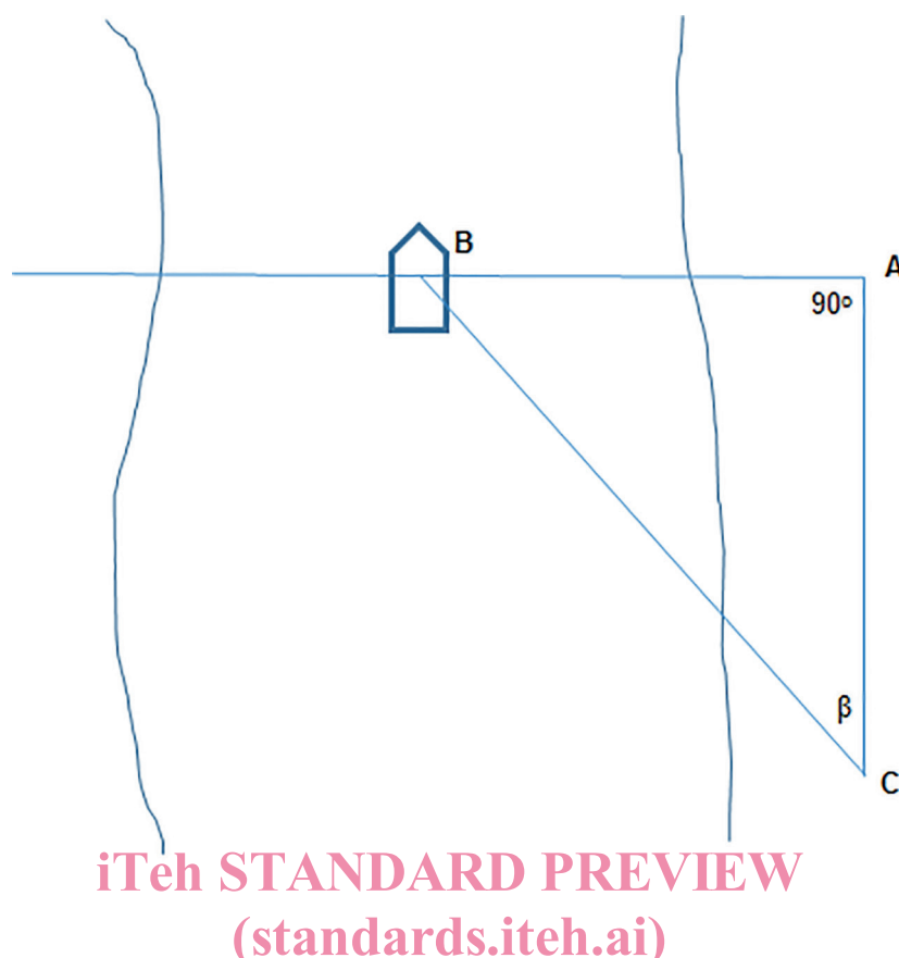
Figure 1 — Position fixing on a cross section by angular techniques
