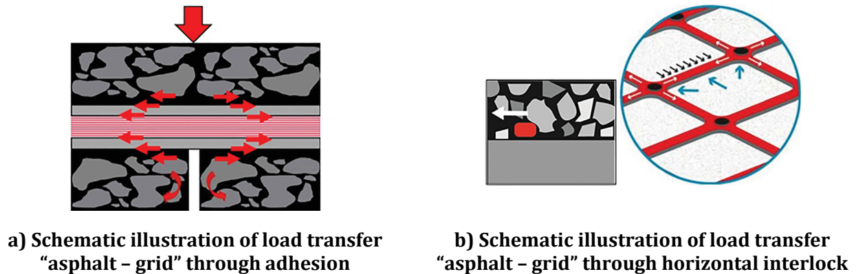
Figure 1— Illustration of load transfer through adhesion and interlock
