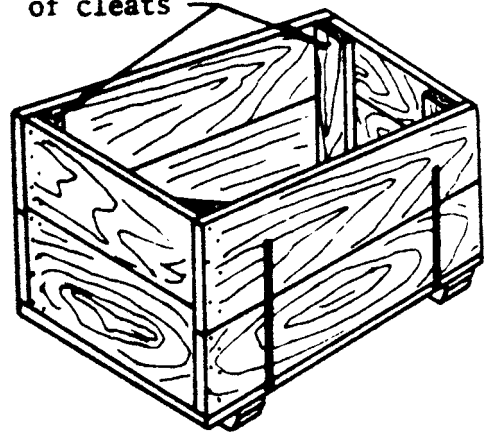
FIG. 4 Style 5 Nail Wood Box A
