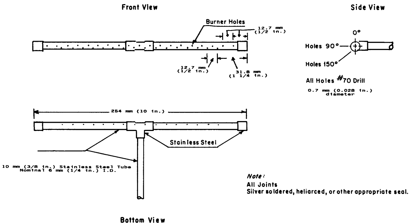
FIG. 5 Pilot Burner
