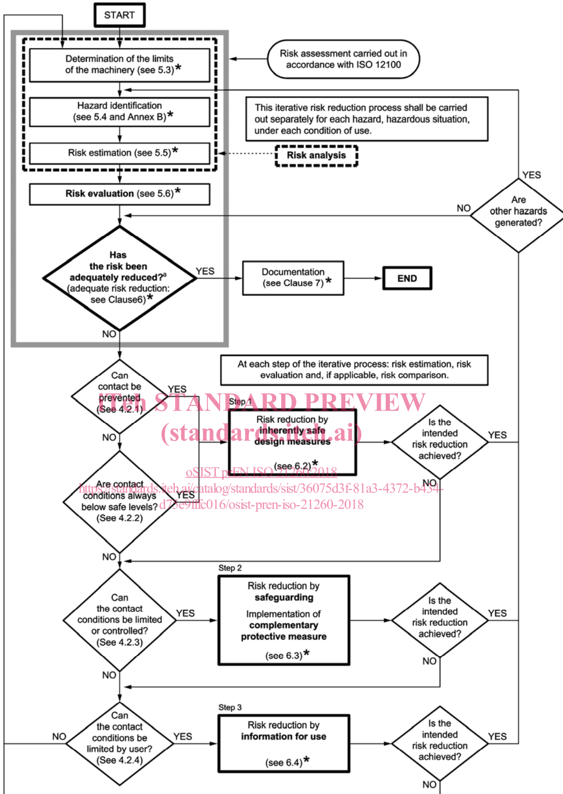
Figure 1 — Overview of risk assessment/risk reduction (see ISO 12100)
