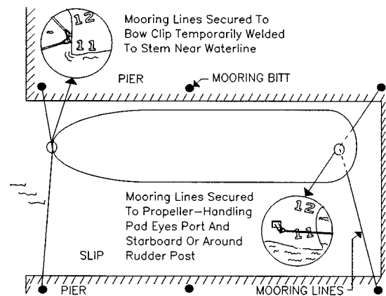
FIG. 11 The Preferred Mooring Arrangement
