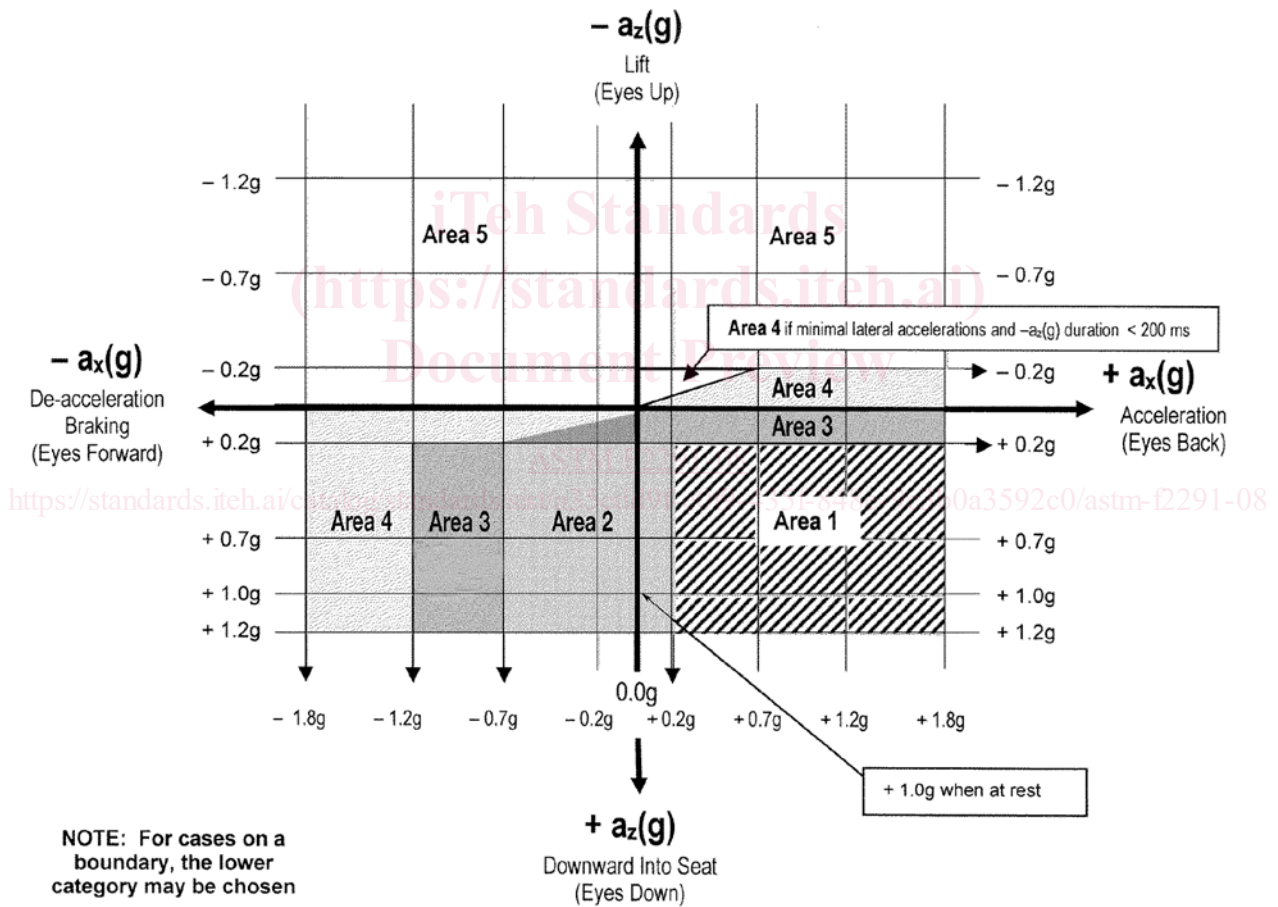
Distinctive Areas 1 through 5 FIG. 2 Restraint Determination Diagram—Accelerations in Design Stage
